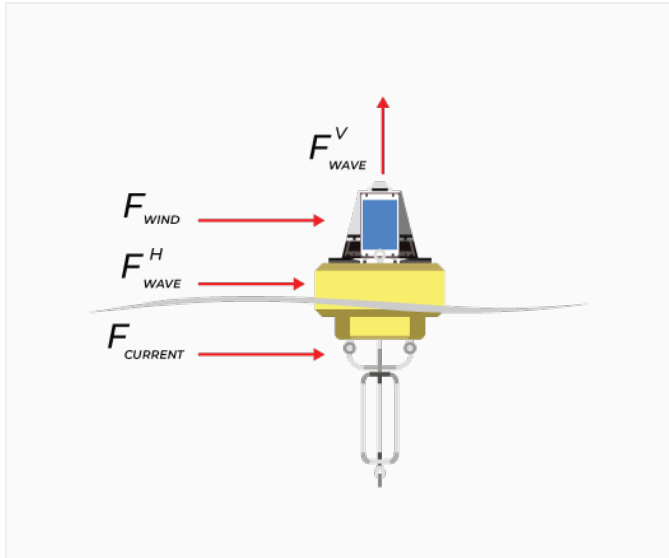
Figure 3: Force diagram representing external forces acting on buoys in natural environments.
