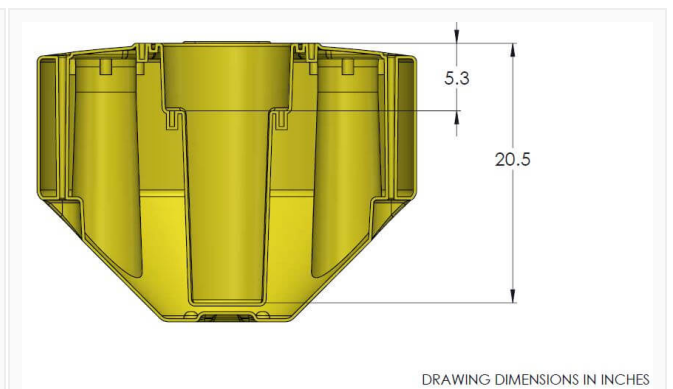
Figure 5: Empty XB-200 battery well.
