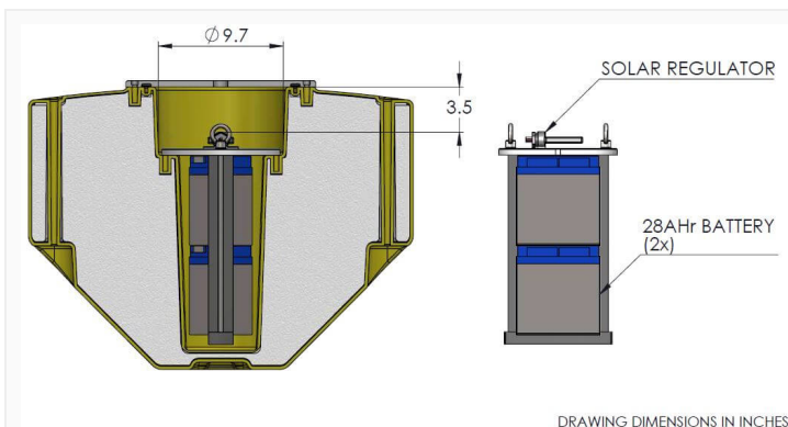
Figure 4: Two 28 Ahr batteries installed.
