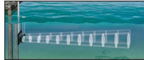
Argonaut-SL in the Field
